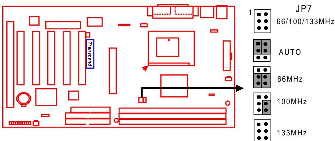
66/100/133MHz FSB Configuration Jumper
