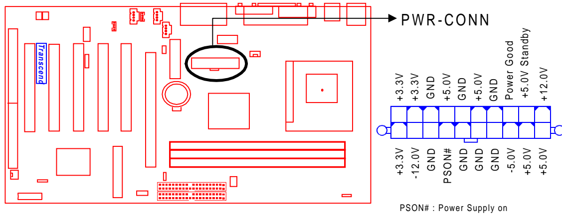
Power Connector
