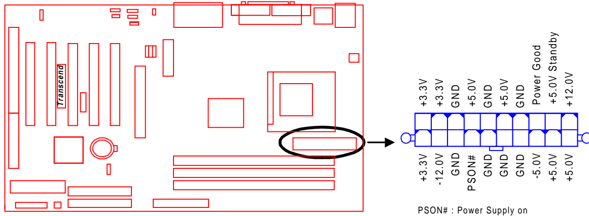
Power Connectors
