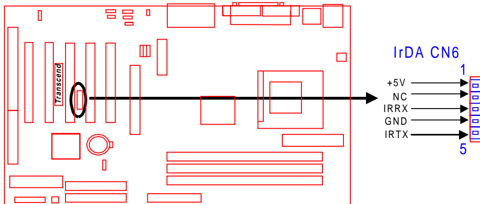
IrDA Connector
