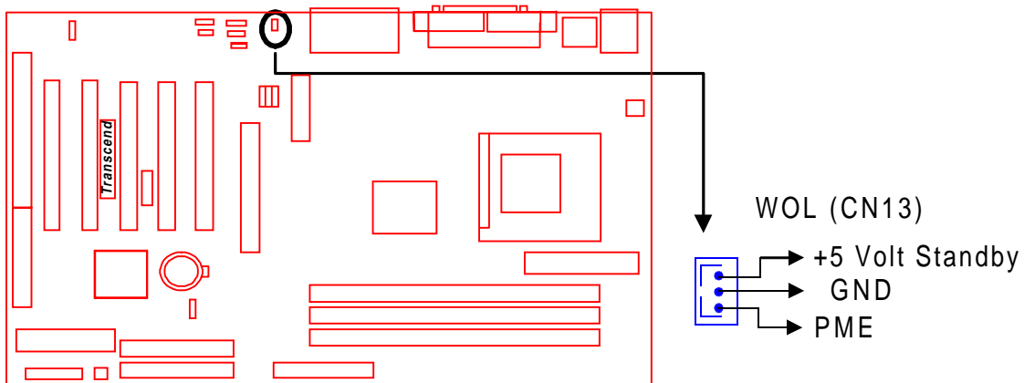
Wake-On-LAN Connector
