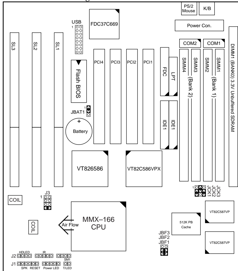
Figure 1-1. SL-53D5-S Motherboard Layout
