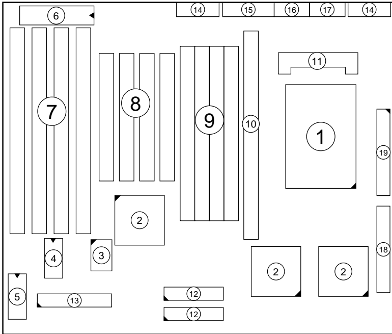
Figure 1-1. Mainboard Layout
