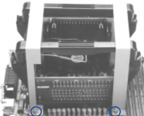
Retention mechanism frame around single processor configuration with terminator.
