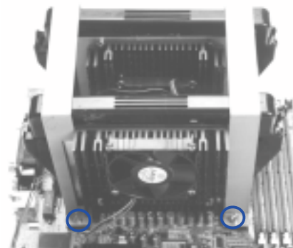
Retention mechanism frame around dual processor configuration.
