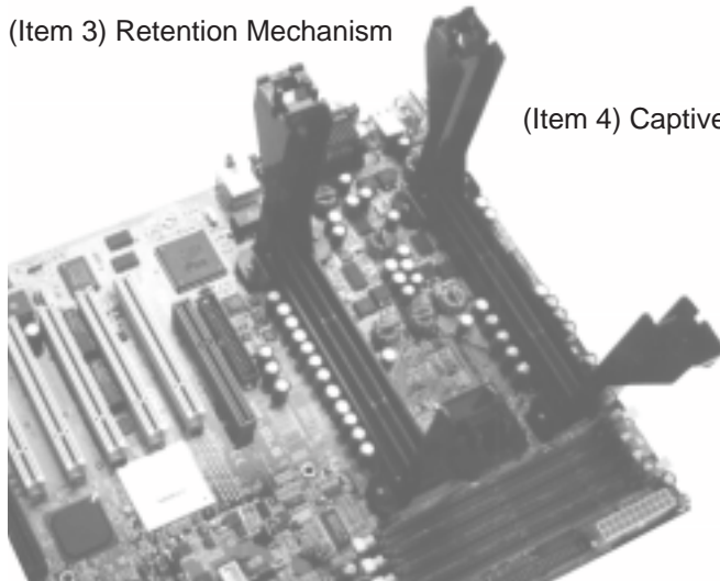
Two retention mechanisms installed
