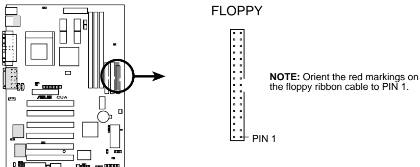
CUA Floppy Disk Drive Connector
