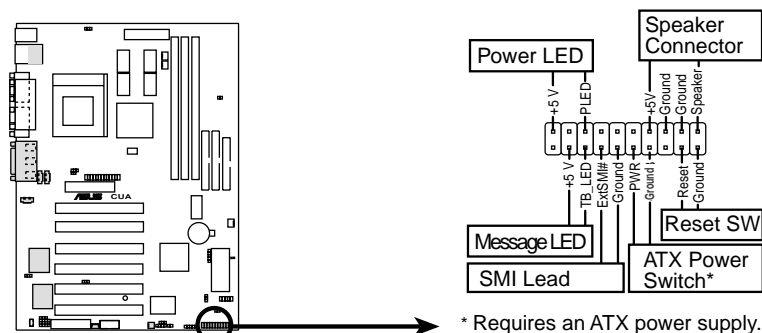
CUA System Panel Connectors
