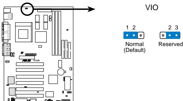
CUA Input/Output Voltage Setting
