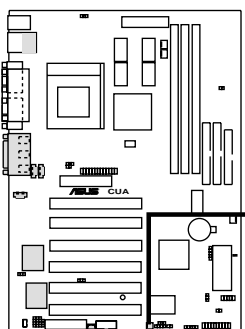
A7V Wake-On-Ring Connector
