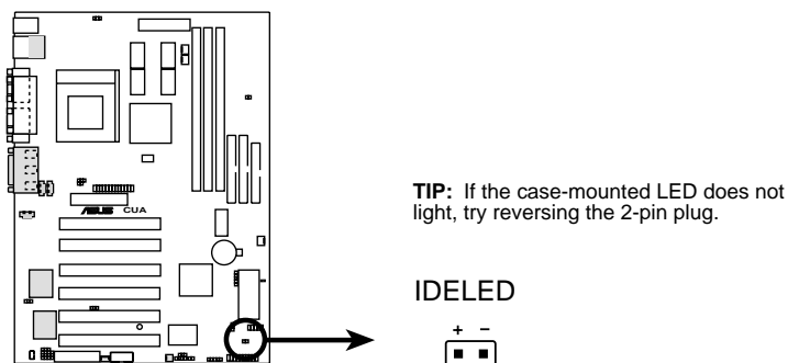
CUA IDE Activity LED
