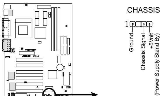
CUA Chassis Open Alarm Lead
