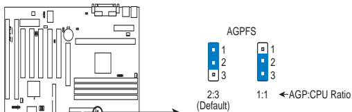
P2B-F AGP Settings
