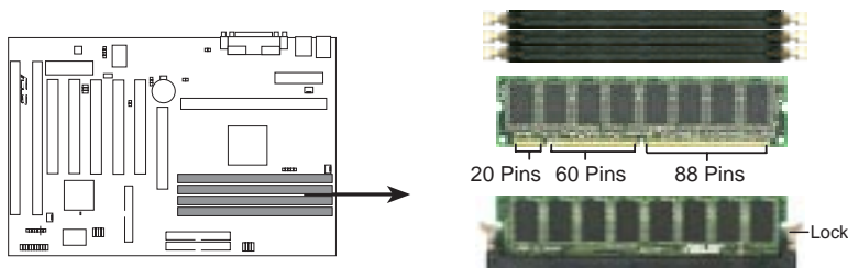
P2B-F 168-Pin DIMM Memory Sockets
