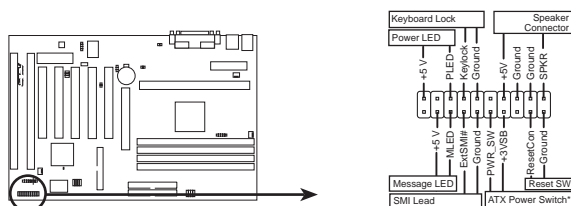
P2B-F System Panel Connections
