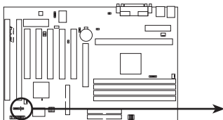
P2B-F IDE Activity LED
