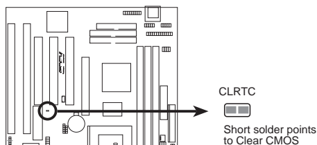
P5A-B Clear RTC RAM
