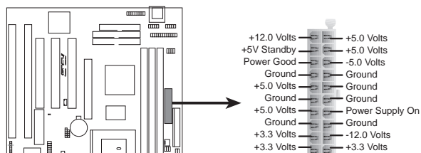
P5A-B ATX Power Connector
