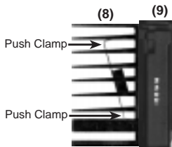
SEC Cartridge with Heatsink (Side View)
