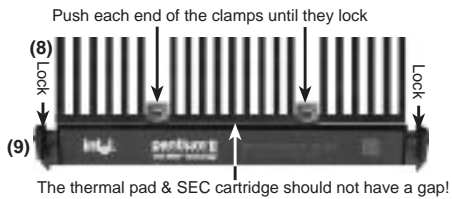
SEC Cartridge with Heatsink (Top View)
