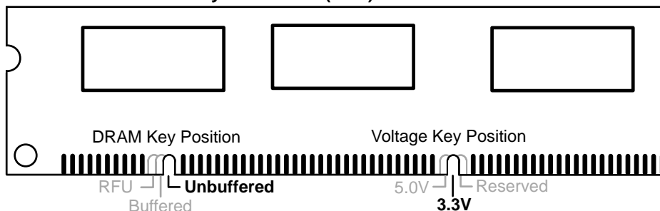
A7A266 168-Pin SDR DIMM Sockets
