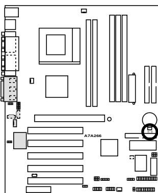
A7A266 Clear RTC RAM
