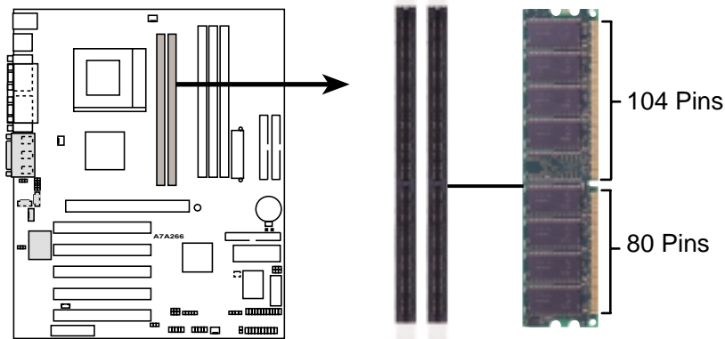
A7A266 184-Pin DDR DIMM Sockets
