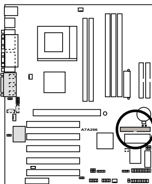
A7A266 Floppy Disk Drive Connector
